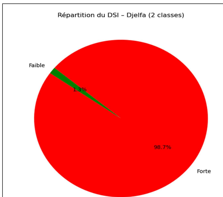
Figure 49: Répartition du DSI pie chart Djelfa
