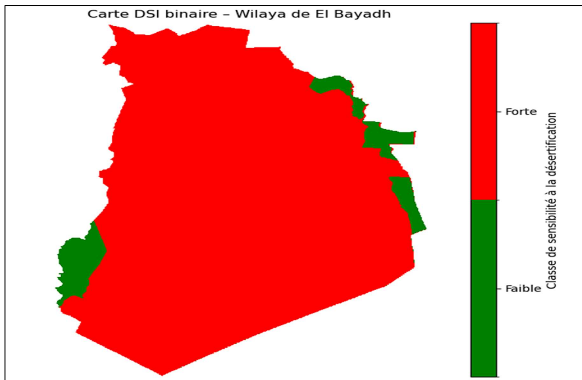
Figure 50: Carte DSI Wilaya Elbayadh
