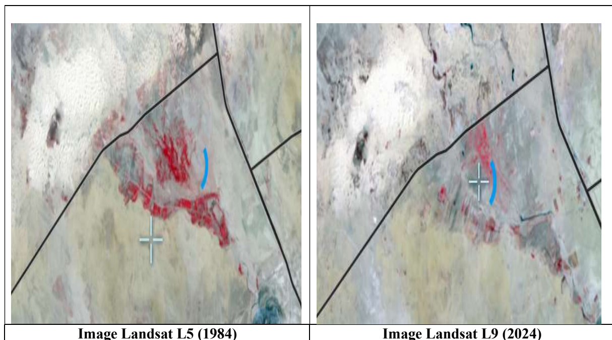
Figure 21: Image Landsat L5 (1984) ET L9 (2024)
