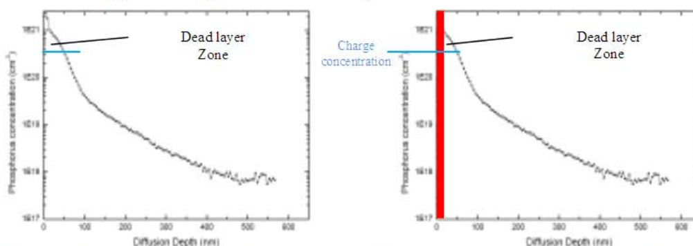
Figure 1: Principle of dead layer reduction by a pre-oxidation step before phosphorus diffusion.
