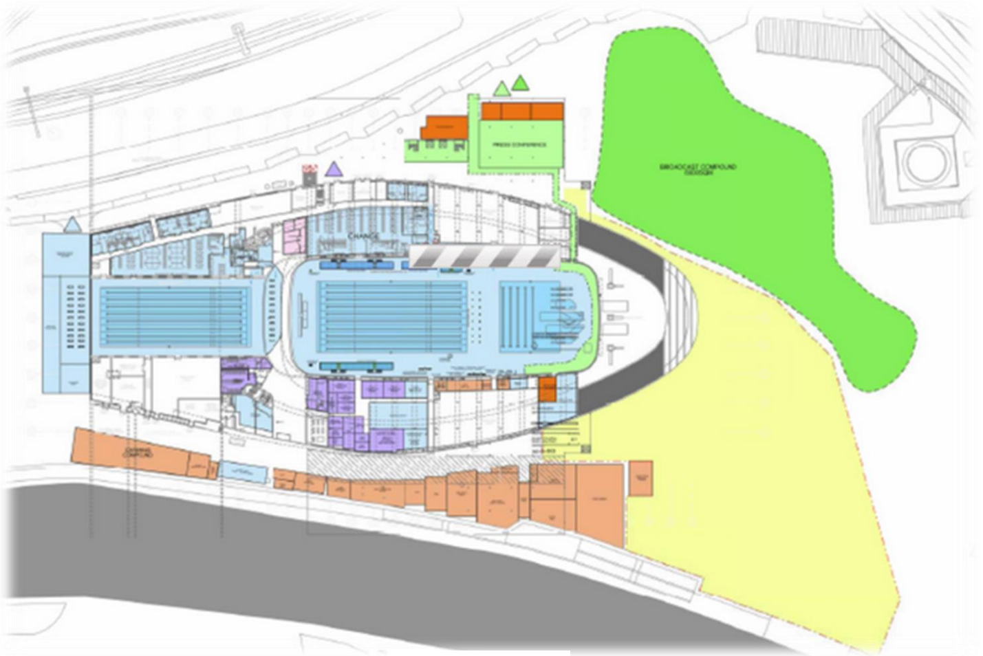
Fig48. Plan RDC
