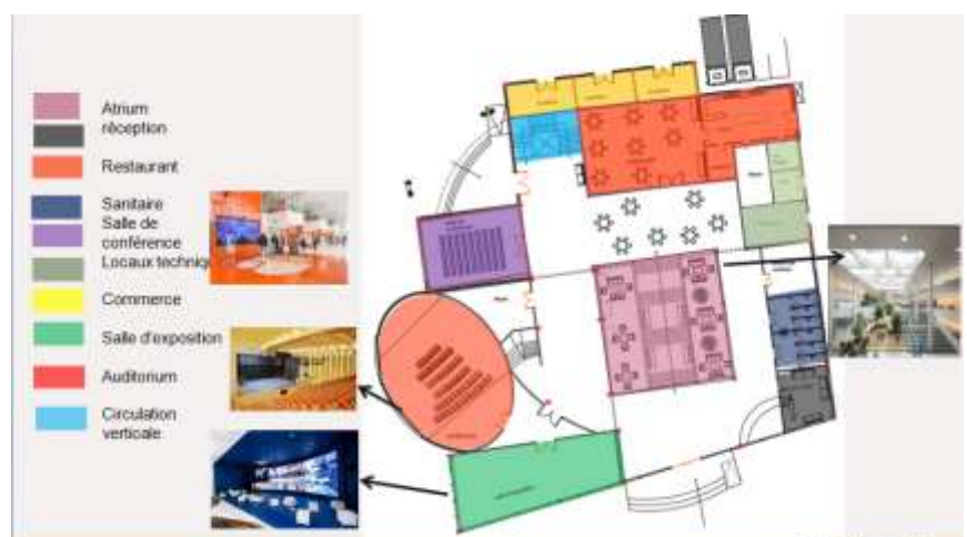
Figure 79PLAN RDC 1/200
