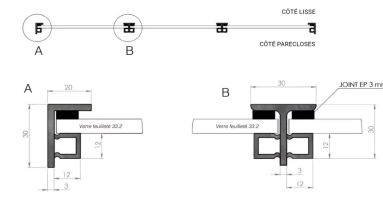
detail verrierre
