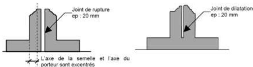
Figure 90 joint de rupture
