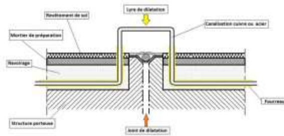
Figure 89 joint de dilatation
