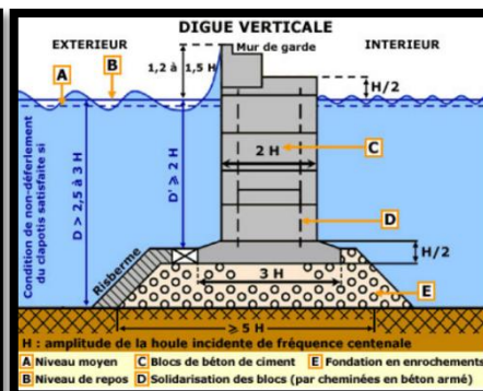
Figure 212: digue vertical
