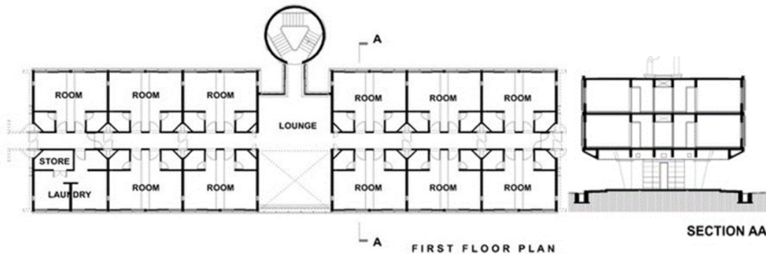
Figure 44: coupe transversale
