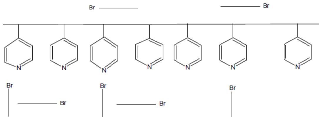
Figure III.9: Greffage aléatoire
