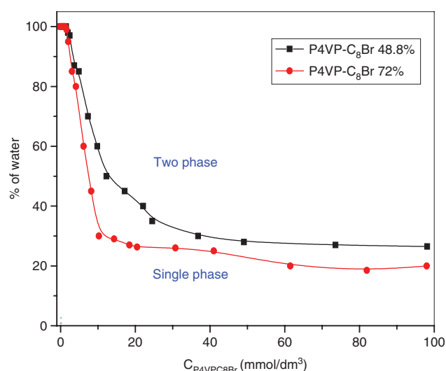
Figure 1: Phase diagram of the P4VPC 8 Br 72% and P4VPC 8 Br 48.8% on the solubility at 25^\circ\text{C} in the mixture of water-ethanol.
