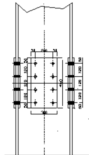
Figure VII.3 : Assemblage poteau-poteau
