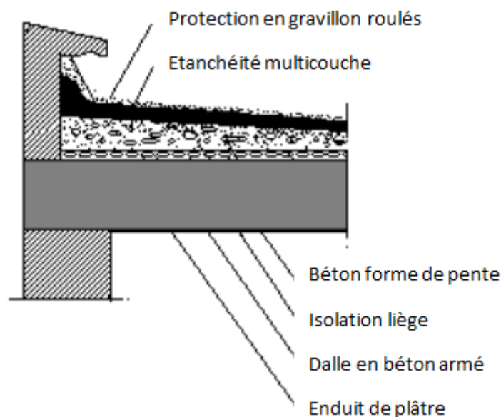
Figure II.1 : plancher terrasse.
