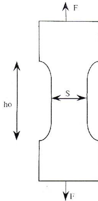
Figure 1 Traction uniaxiale
