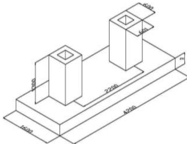
Figure (7.2) : Semelle filante
