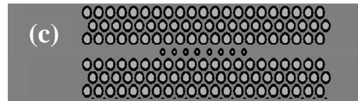
Fig. 3 Resonant band-pass filters realized by cascading Fabry-Pérot (FP) cavities in a one-missing-row PhC waveguide. (a) Three cavities are used utilizing 4 extra rods, (b) five cavities are used utilizing 6 extra rods, (c) Seven cavities are used utilizing 8 extra rods.
