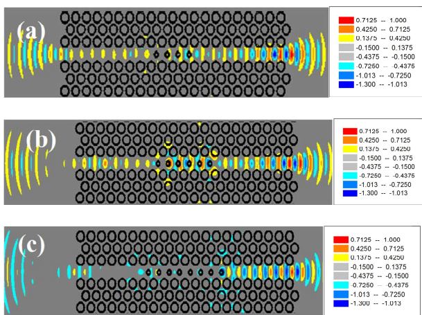
Fig. 6 The distribution shape of the magnetic field Hz excited in TE mode, \Delta x = \Delta y = 0.04 \mu\text{m} . (a) Three cavities are used utilizing 4 extra rods, (b) five cavities are used utilizing 6 extra rods, (c) Seven cavities are used utilizing 8 extra rods.
