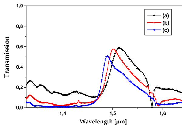
Fig. 4 Normalized transmission spectra obtained by the two-dimensional finite difference time domain (2D FDTD) simulation for the structure illustrated in fig. 3.
