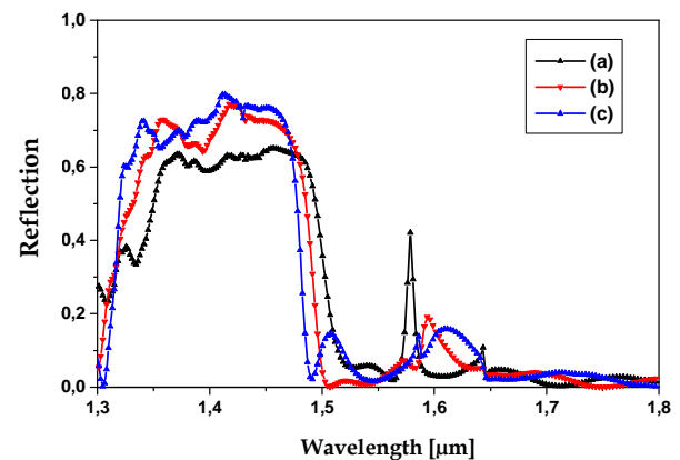
Fig. 5 Normalized reflection spectra obtained by the two-dimensional finite difference time domain (2D FDTD) simulation for the structure illustrated in fig. 3.
