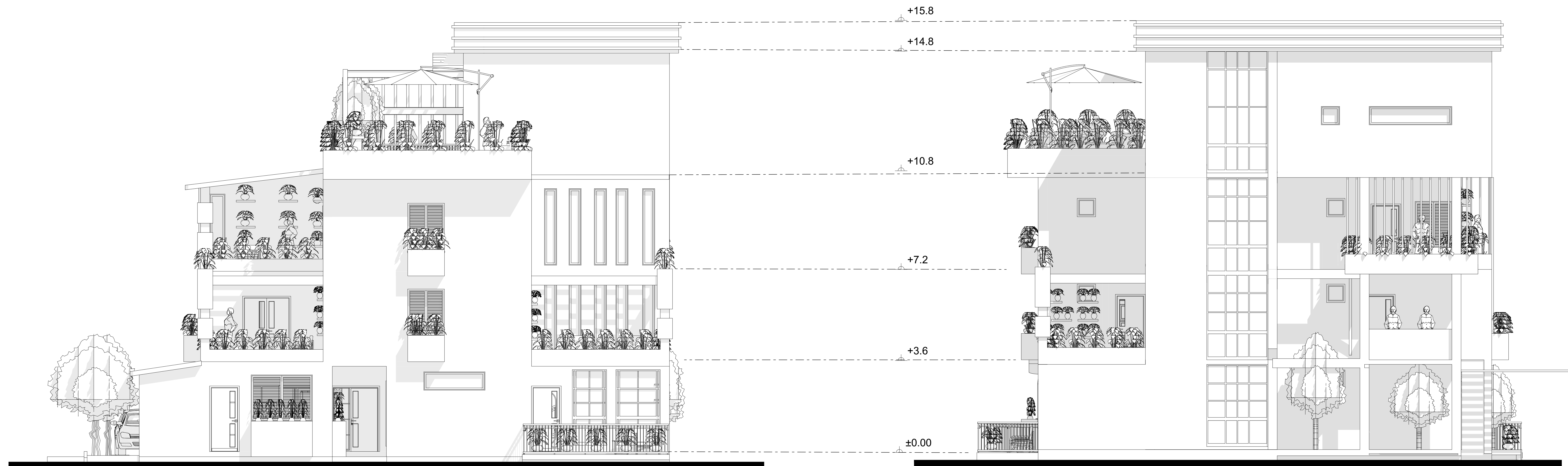
Left side Elevation
