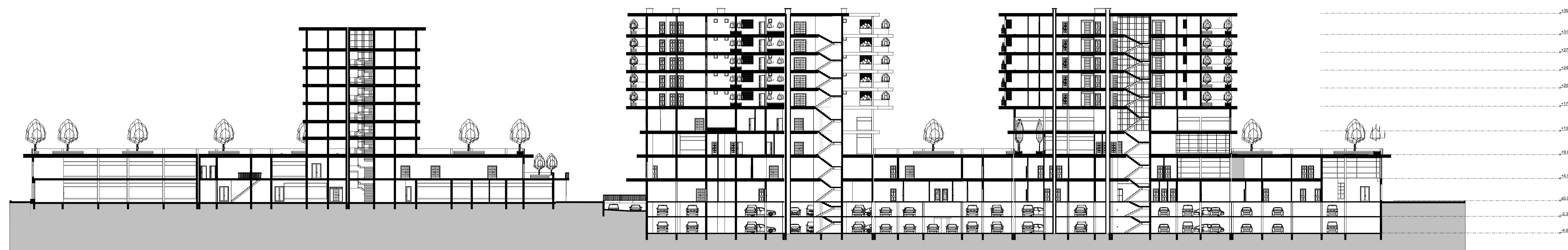
SECTION A-A OF COLLECTIVE HOUSING
