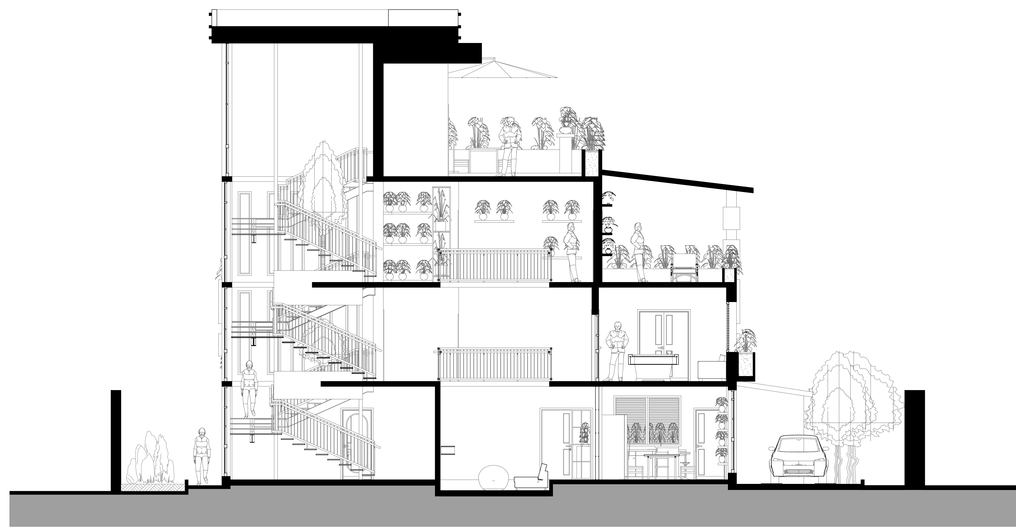
SECTION AA
