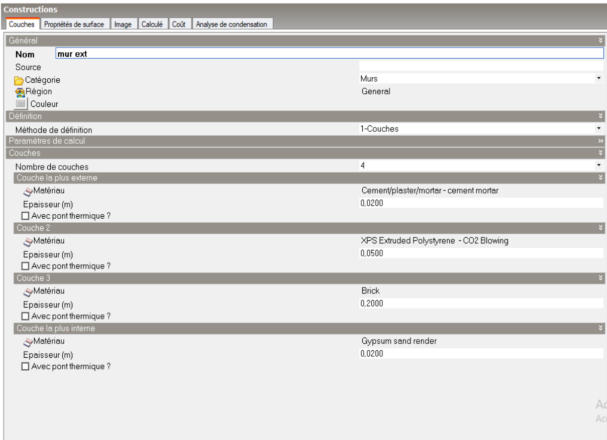
Figure 41 : Opaque construction built up by layers
