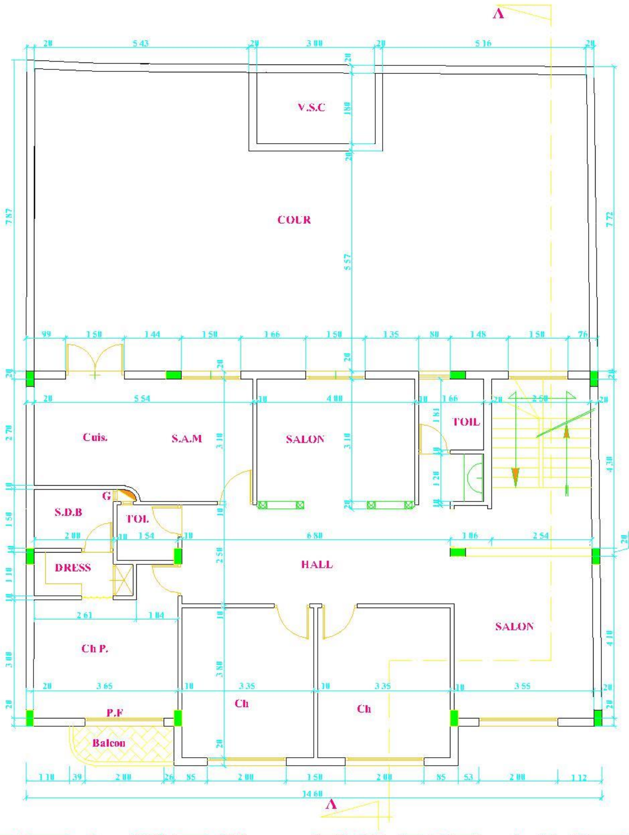
Figure 32 : floors plan
