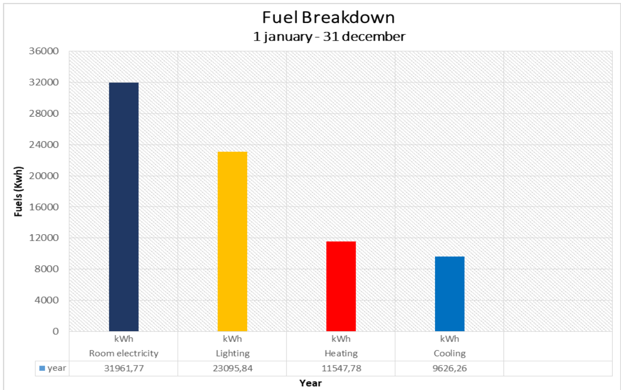
Figure 48 : Graph (a) : variety of combustibles without insulation
