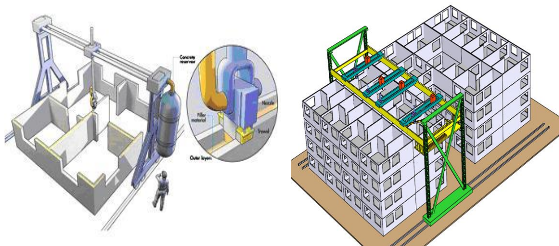
Figure 2.14 : imprimantes 3D Contour Crafting [27]
