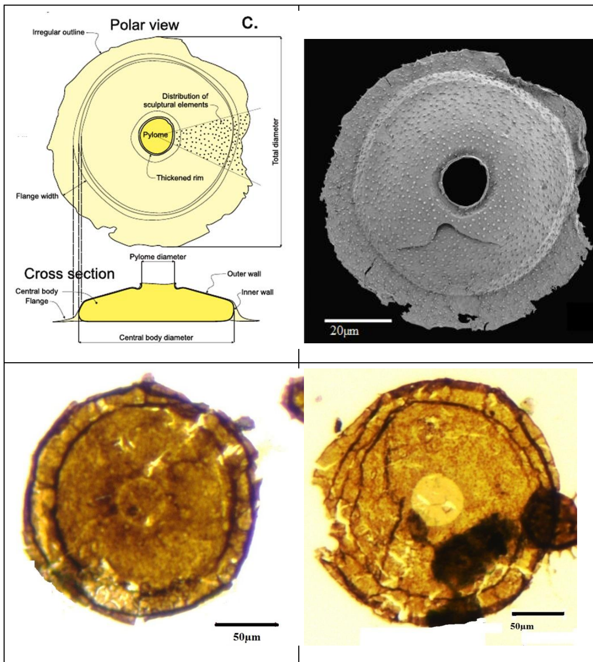
Fig. 4. 1, 2; Halodinium verrucatum Gurdebeke et al. (2018, fig. 2C, fig. 4a) 3,4; Saharidia fragilis Combaz 1967
