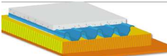
Figure 111 : plancher collaborant 41
