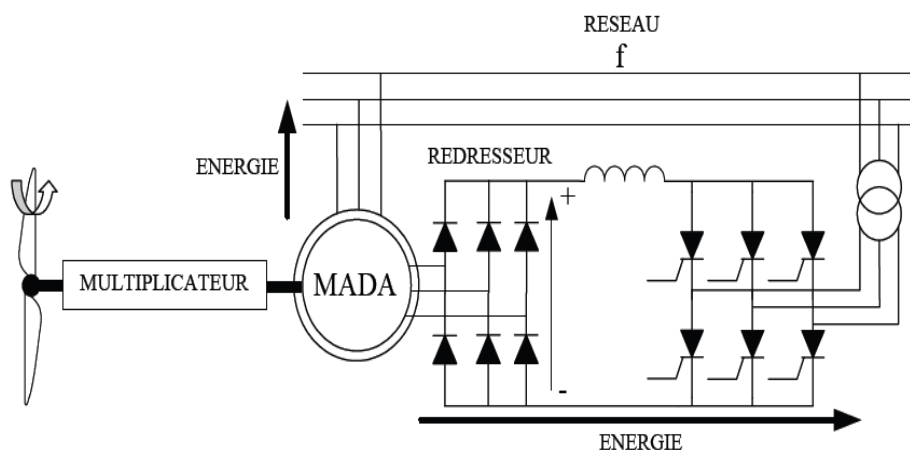
Figure. I.20.MADA structure Kramer [12]
