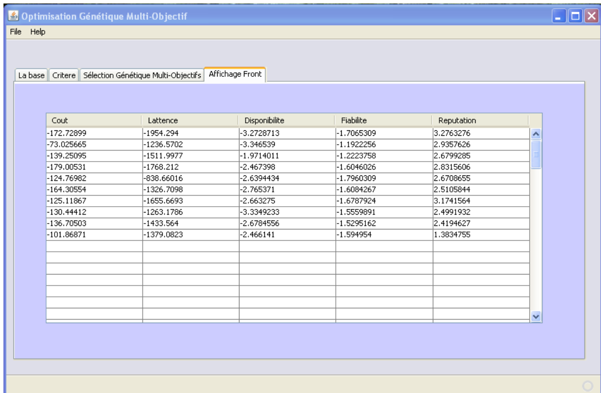
Figure III.7 affichage du front de Pareto final
