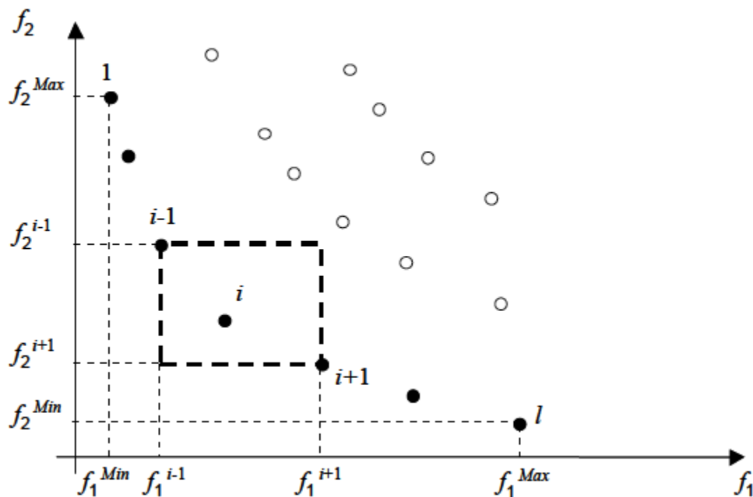
Figure II.9 : Distance de crowding (Distance de surpeuplement)
