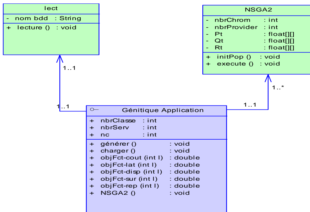
Figure III.3 Diagramme de classe
