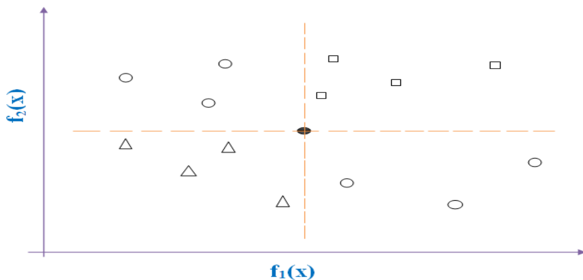
Figure II.1 Exemple de dominance
