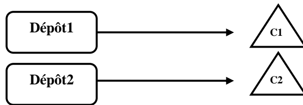
Figure 1.6 : Distribution un-vers-un
