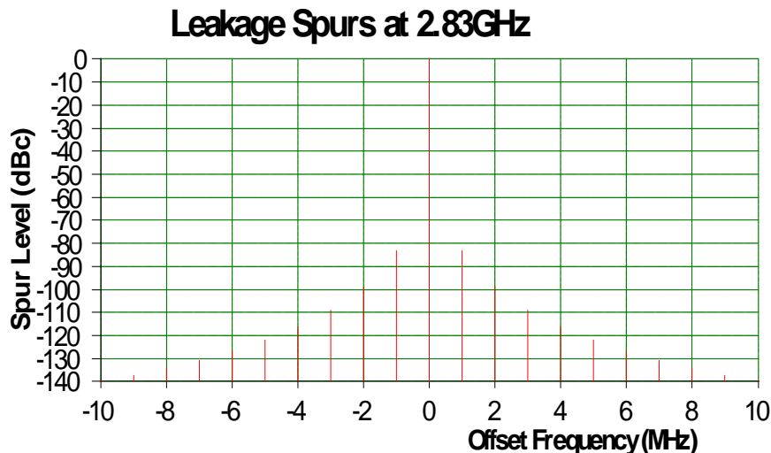
Figure IV.4. Leakage spurs.
