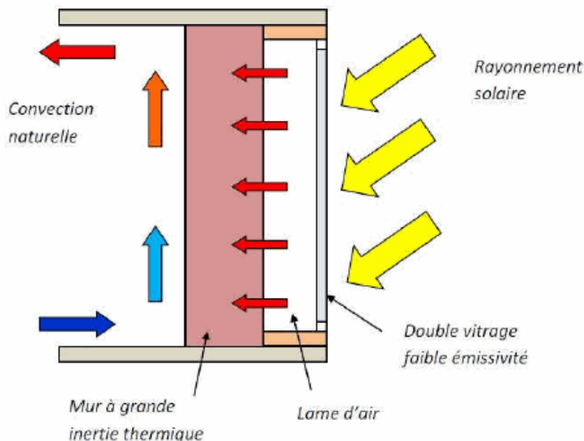
Figure 61: Façade active
