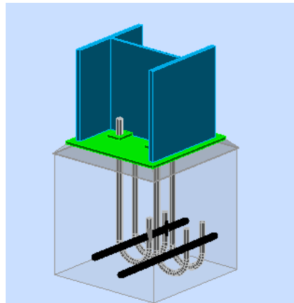
Figure VI.6 Assemblage pied de poteau
