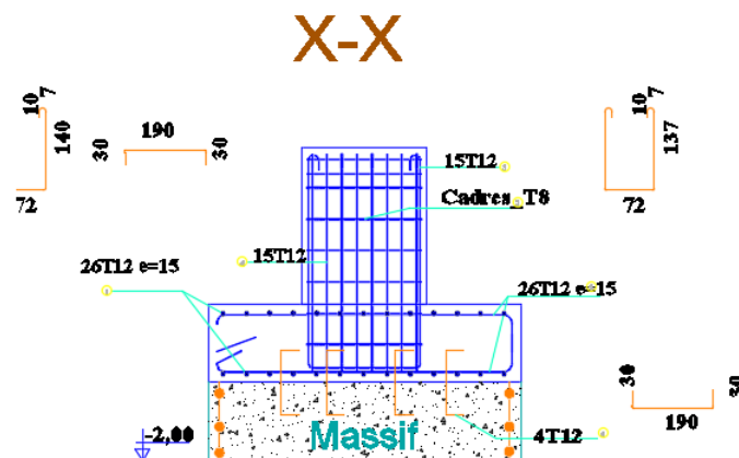
Figure VII.2: Ferrailage de la semelle
